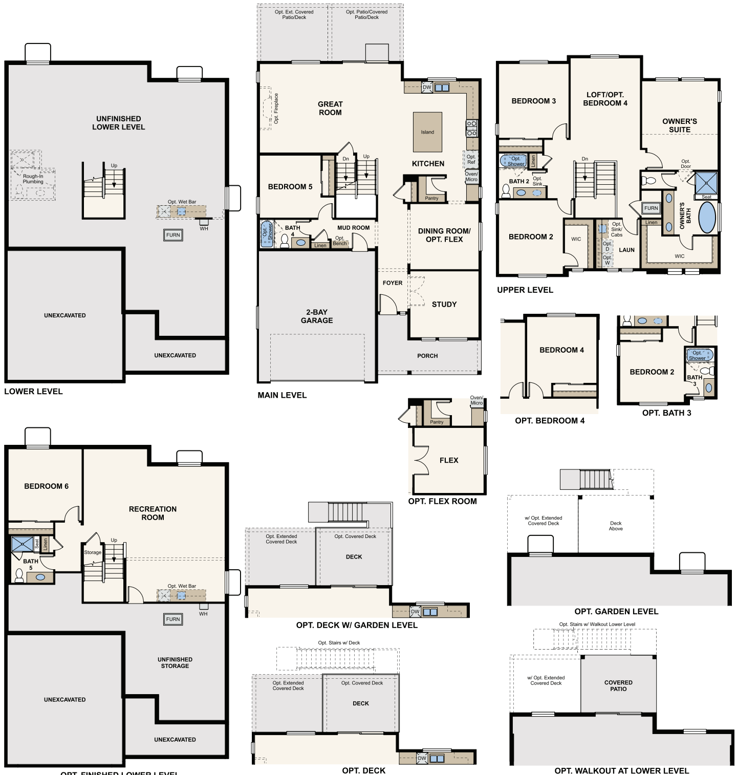
FLOOR PLAN
